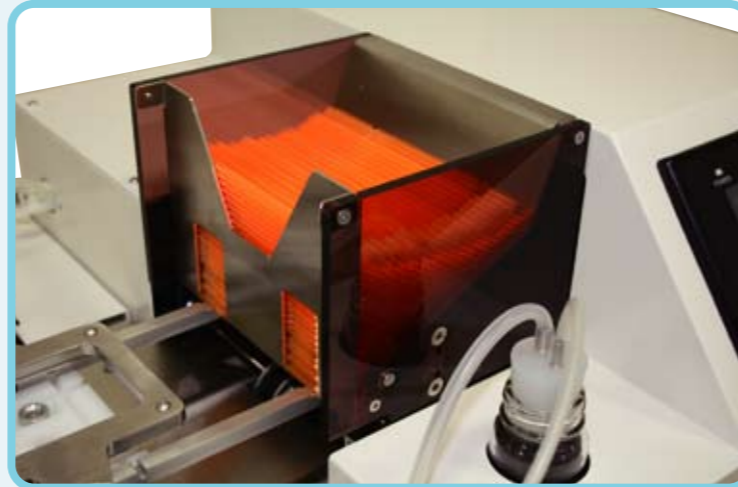
Straw hopper with capacity 650pcs (0.5ml straws)
