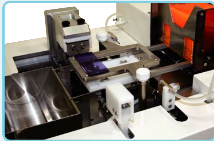
Filling and sealing station
